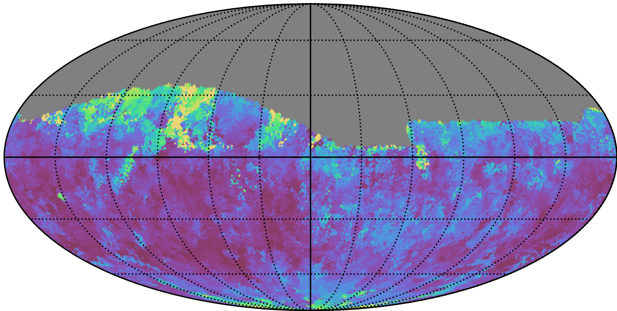
early_u_fpextra4.0_v3.4_10yrs Yr 1 z band: Median seeingEff
