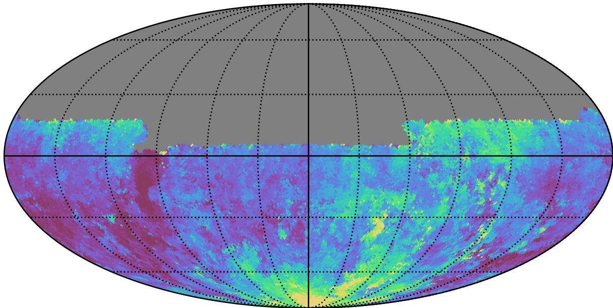
early_u_fpextra4.0_v3.4_10yrs Yr 1 u band: Median seeingEff
