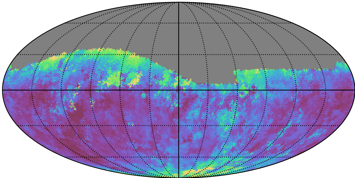
early_u_fpextra4.0_v3.4_10yrs Yr 1 r band: Median seeingEff
