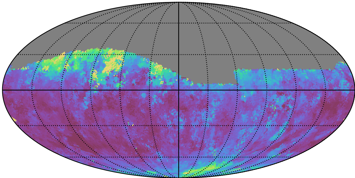
early_u_fpextra4.0_v3.4_10yrs Yr 1 i band: Median seeingEff
