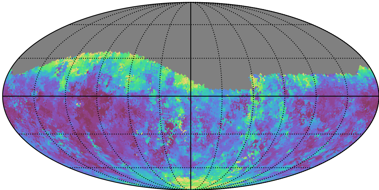
early_u_fpextra4.0_v3.4_10yrs Yr 1 g band: Median seeingEff
