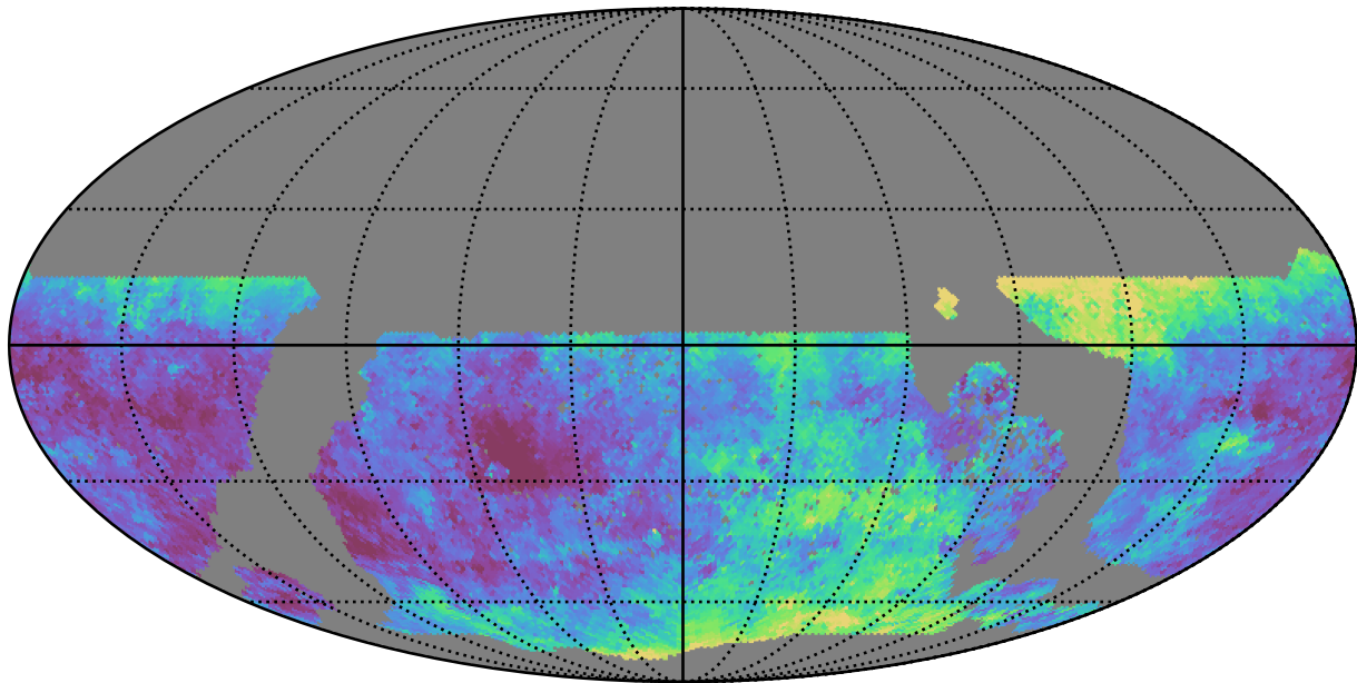
early_u_fpextra4.0_v3.4_10yrs WFD u band: Median seeingEff
