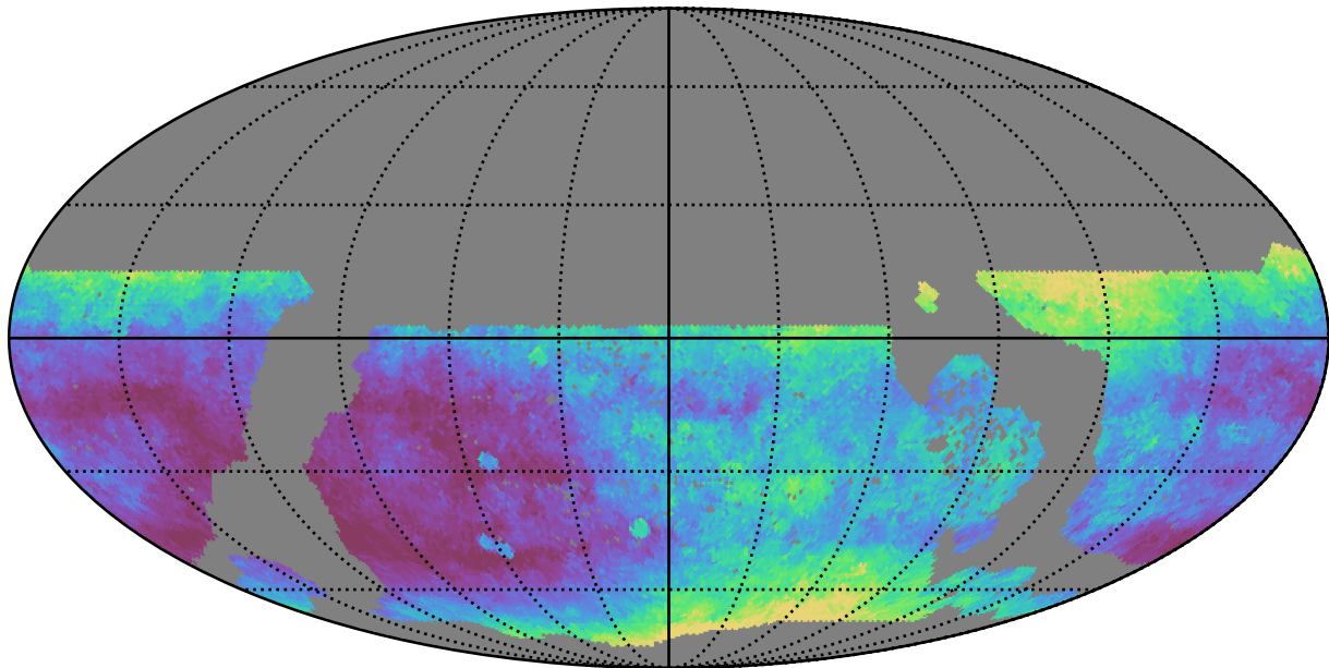
early_u_fpextra4.0_v3.4_10yrs WFD i band: Median seeingEff
