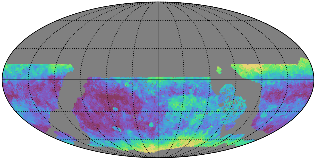
early_u_fpextra4.0_v3.4_10yrs WFD g band: Median seeingEff
