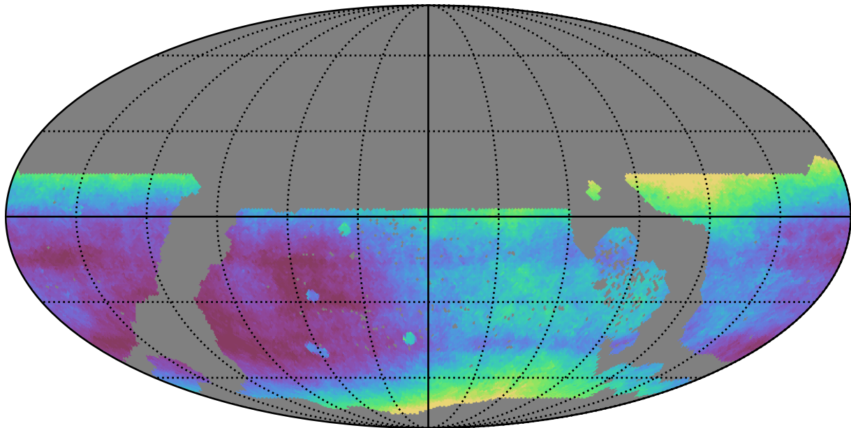
early_u_fpextra4.0_v3.4_10yrs WFD all bands: Median seeingEff
