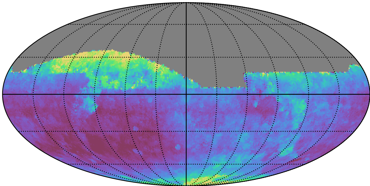
early_u_fpextra4.0_v3.4_10yrs All sky z band: Median seeingEff
