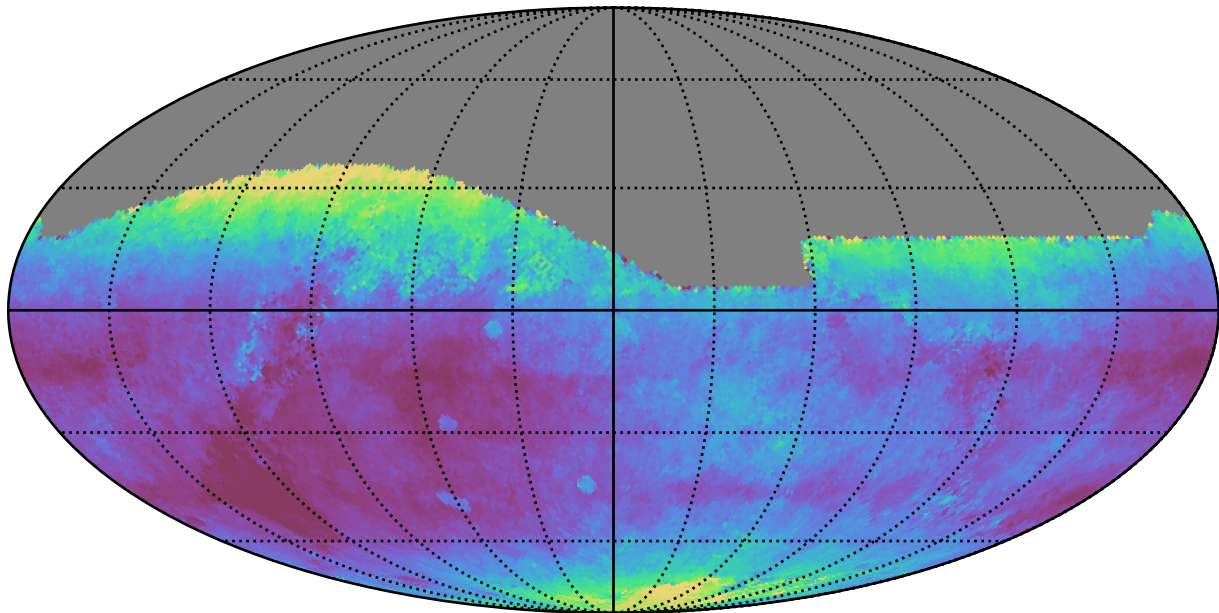
early_u_fpextra4.0_v3.4_10yrs All sky r band: Median seeingEff
