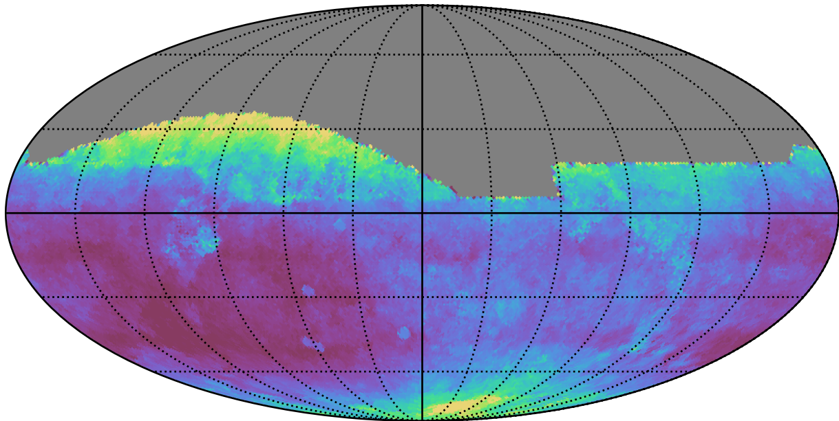
early_u_fpextra4.0_v3.4_10yrs All sky i band: Median seeingEff
