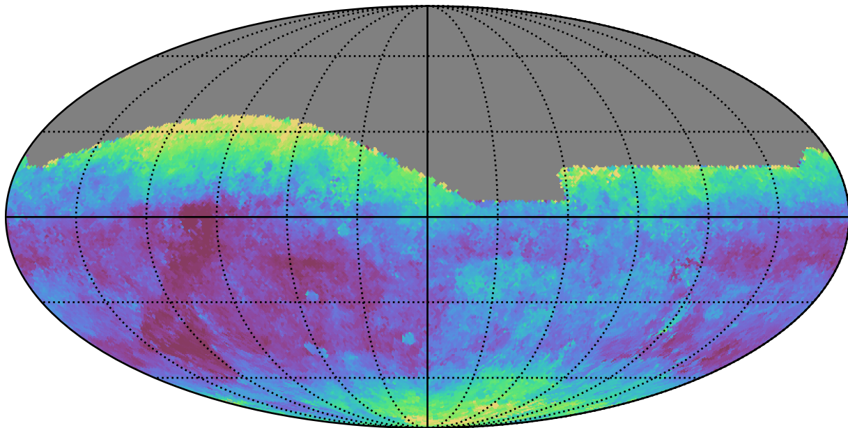
early_u_fpextra4.0_v3.4_10yrs All sky g band: Median seeingEff
