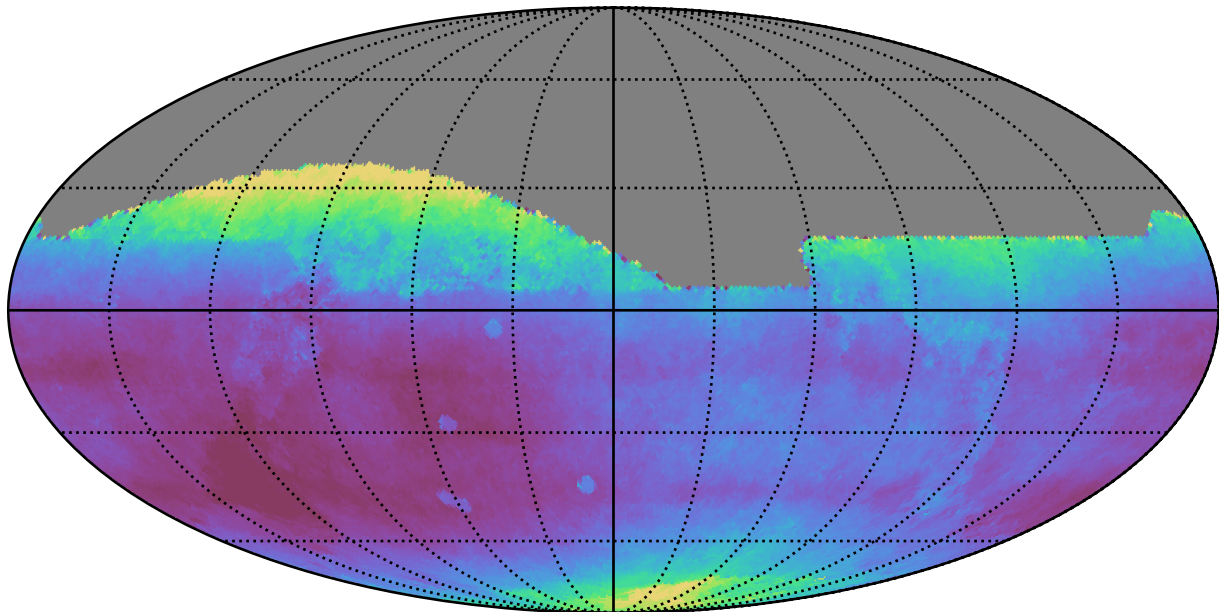
early_u_fpextra4.0_v3.4_10yrs All sky all bands: Median seeingEff
