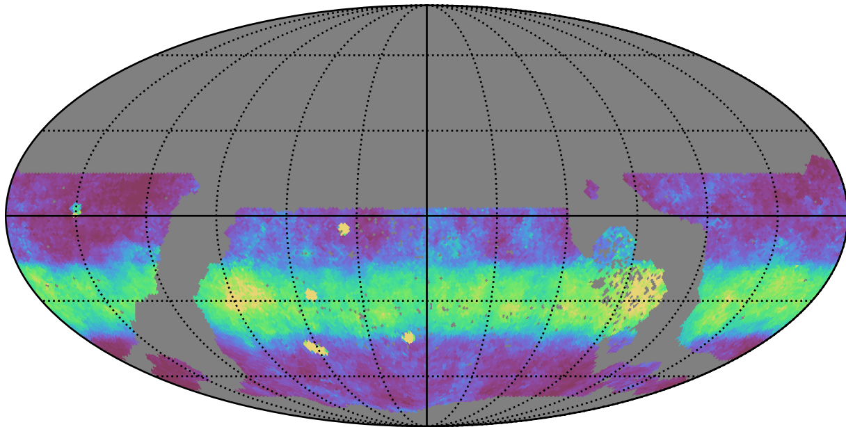
early_u_fpextra4.0_v3.4_10yrs WFD y band: Median normairmass
