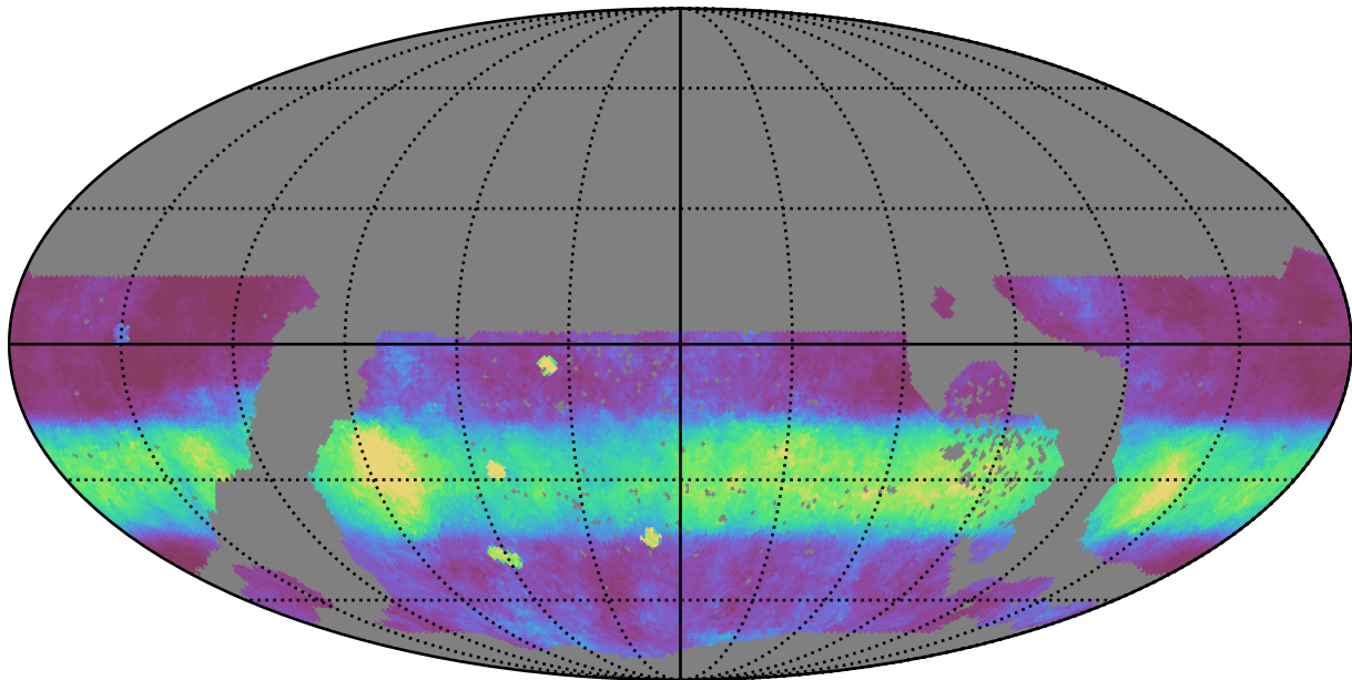
early_u_fpextra4.0_v3.4_10yrs WFD r band: Median normairmass
