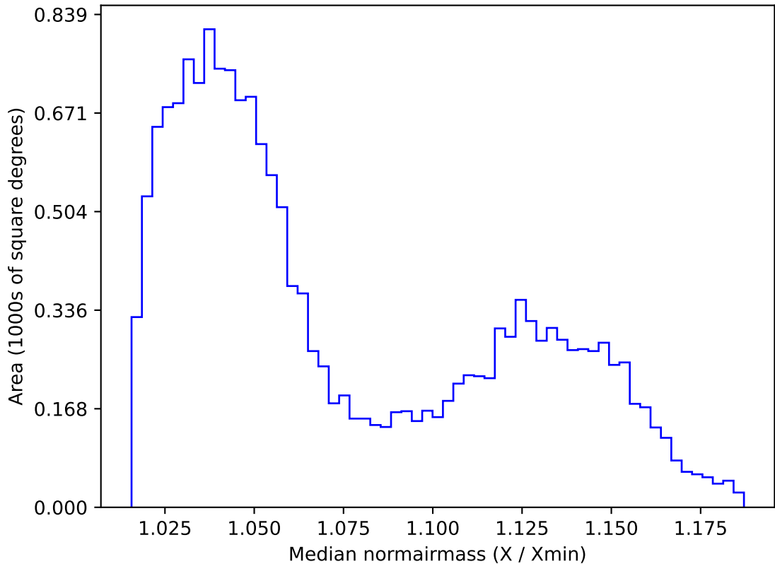
early_u_fpextra4.0_v3.4_10yrs WFD r band: Median normairmass
