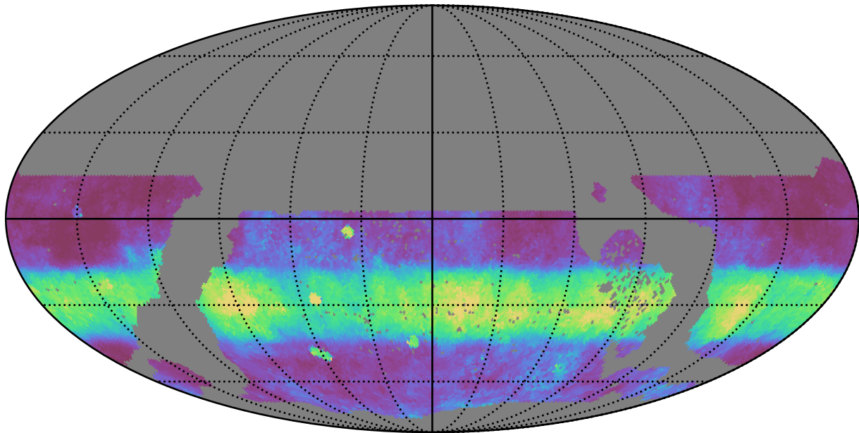
early_u_fpextra4.0_v3.4_10yrs WFD i band: Median normairmass
