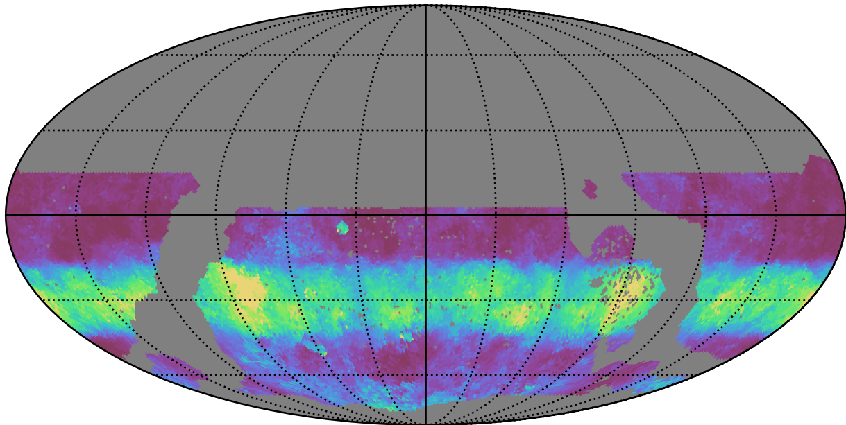
early_u_fpextra4.0_v3.4_10yrs WFD g band: Median normairmass
