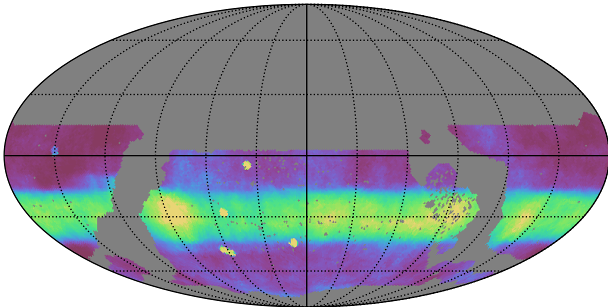
early_u_fpextra4.0_v3.4_10yrs WFD all bands: Median normairmass
