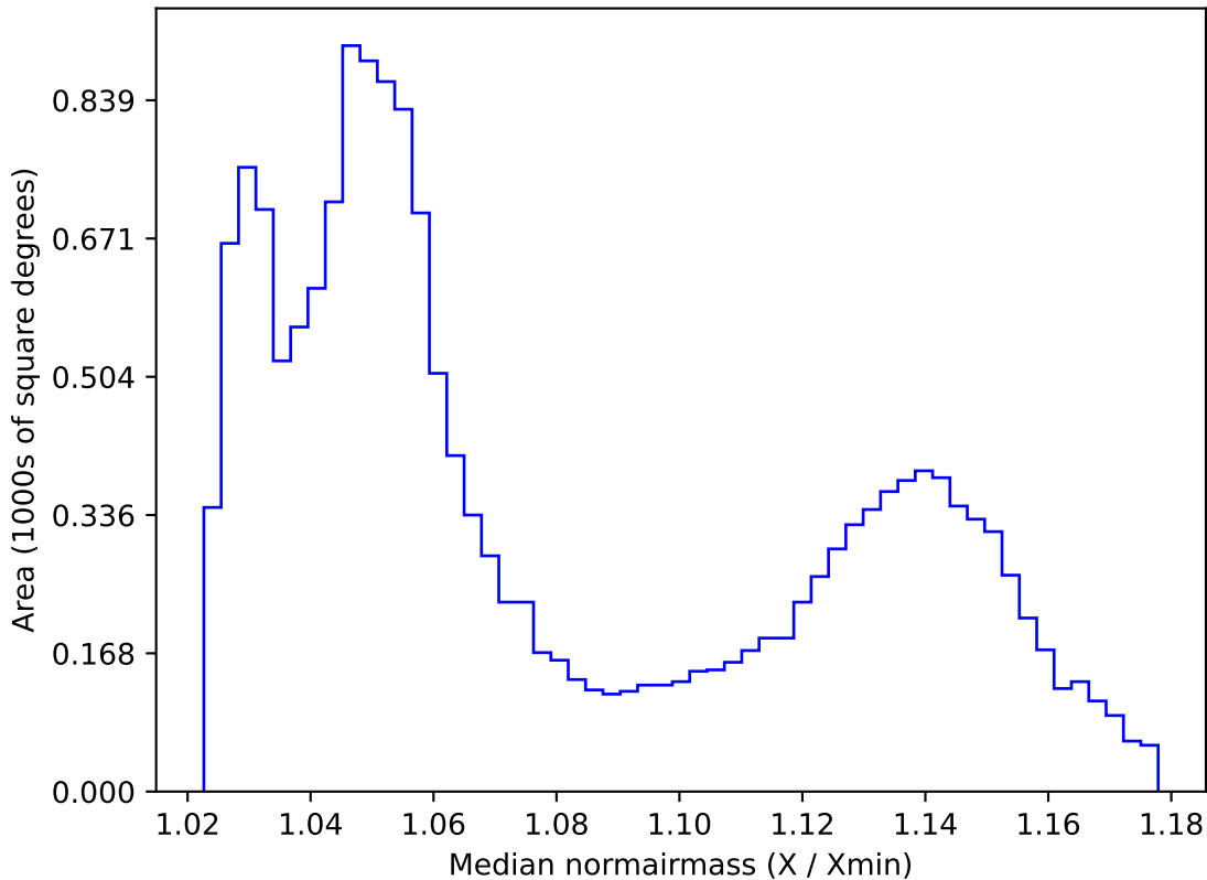
early_u_fpextra4.0_v3.4_10yrs WFD all bands: Median normairmass
