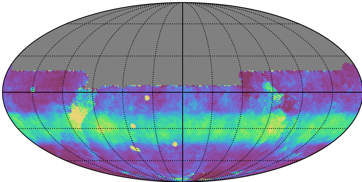
early_u_fpextra4.0_v3.4_10yrs All sky y band: Median normairmass
