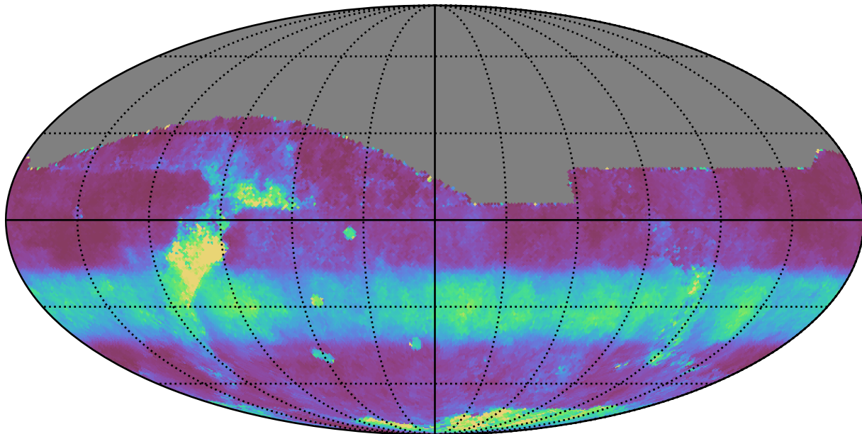
early_u_fpextra4.0_v3.4_10yrs All sky i band: Median normairmass
