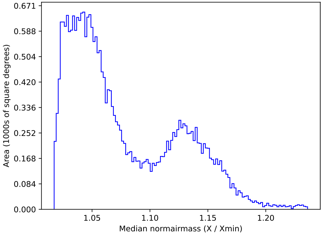
early_u_fpextra4.0_v3.4_10yrs All sky i band: Median normairmass
