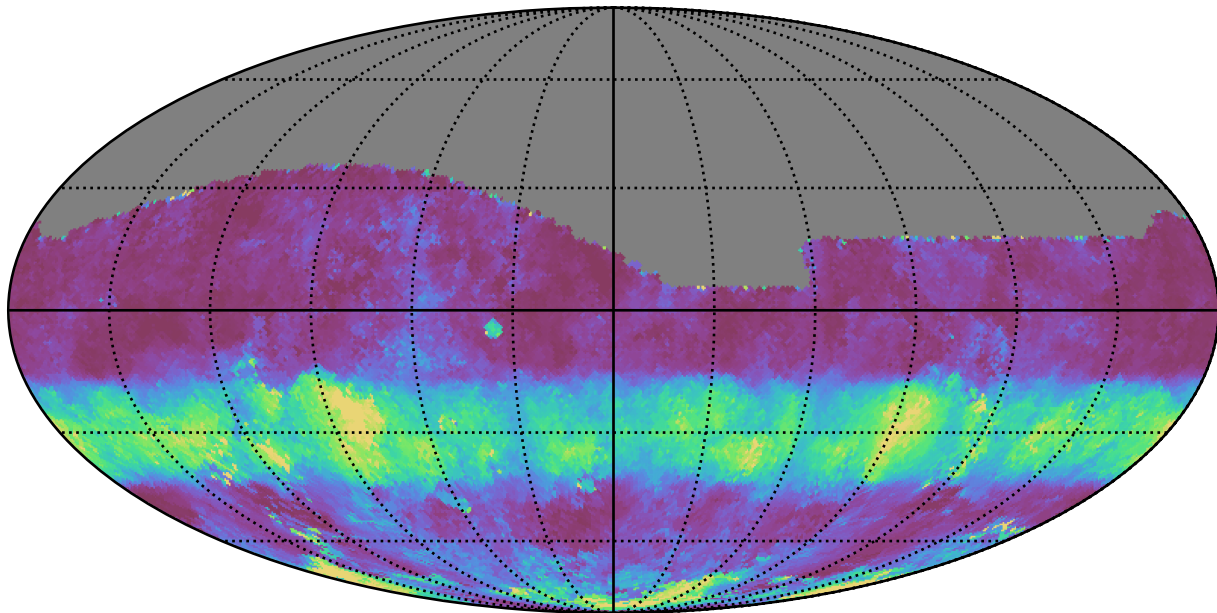
early_u_fpextra4.0_v3.4_10yrs All sky g band: Median normairmass
