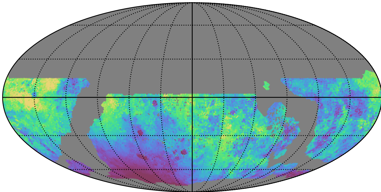
early_u_fpextra4.0_v3.4_10yrs WFD g band: Median moonDistance
