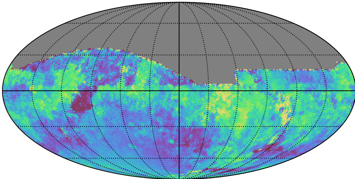
early_u_fpextra4.0_v3.4_10yrs All sky i band: Median moonDistance
