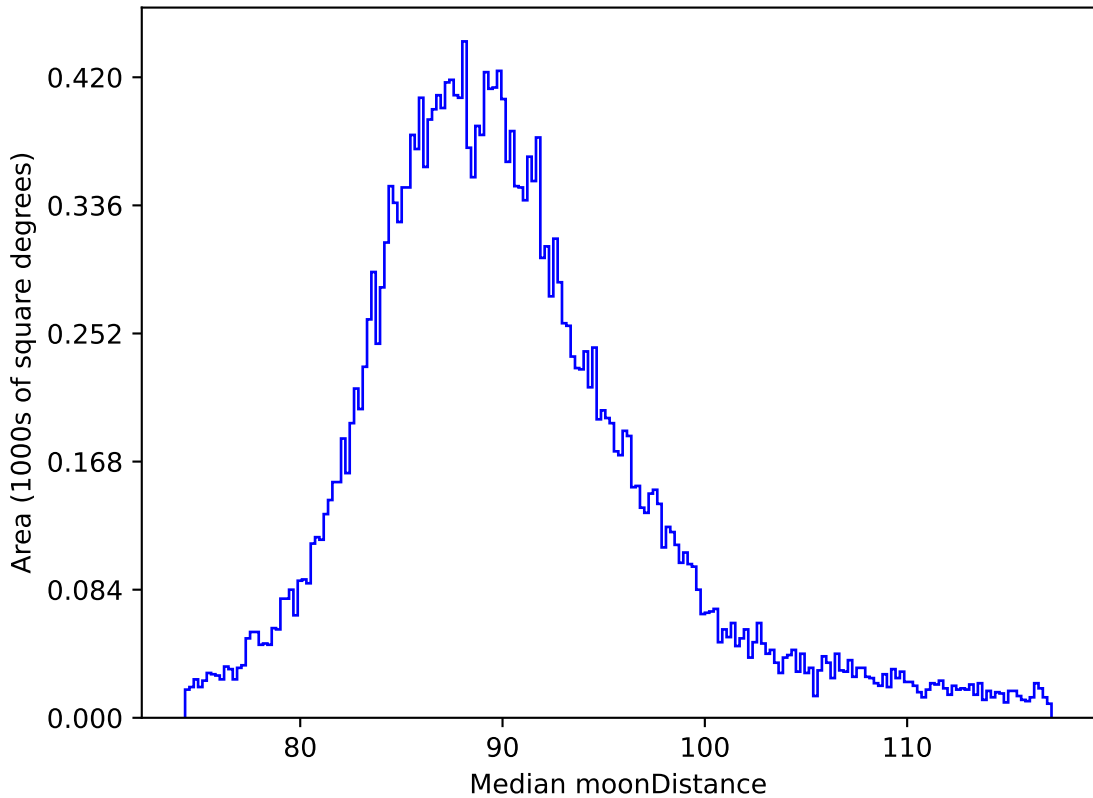
early_u_fpextra4.0_v3.4_10yrs All sky all bands: Median moonDistance
