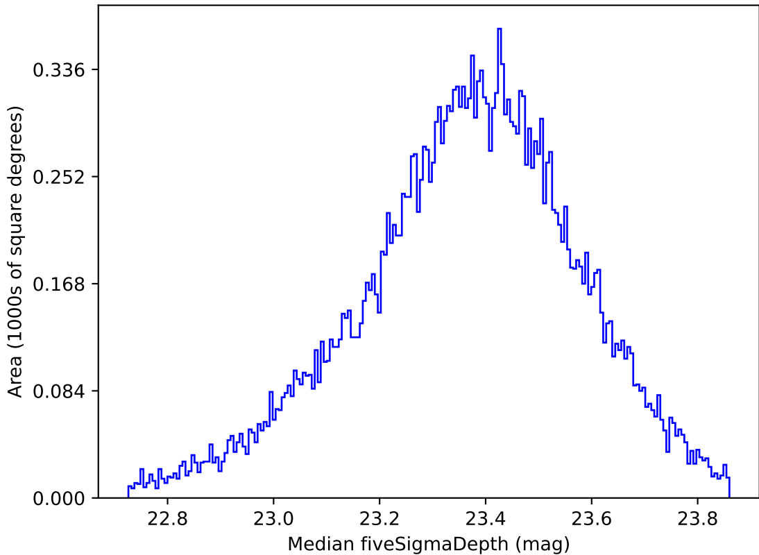
early_u_fpextra4.0_v3.4_10yrs Yr 1 all bands: Median fiveSigmaDepth
