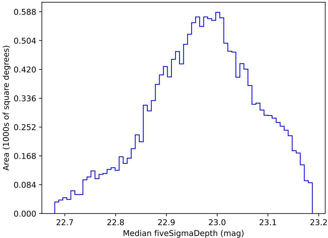
early_u_fpextra4.0_v3.4_10yrs WFD z band: Median fiveSigmaDepth
