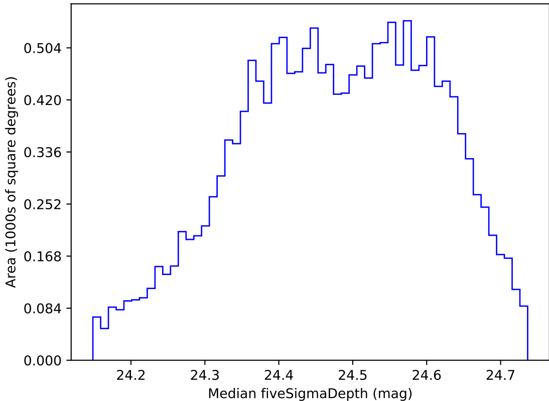
early_u_fpextra4.0_v3.4_10yrs WFD g band: Median fiveSigmaDepth
