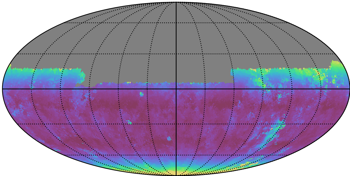
early_u_fpextra4.0_v3.4_10yrs Yr 1 y band: Median airmass
