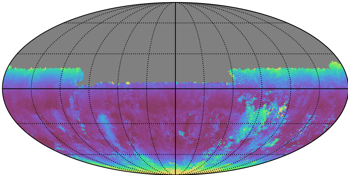
early_u_fpextra4.0_v3.4_10yrs Yr 1 u band: Median airmass
