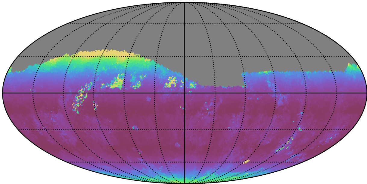
early_u_fpextra4.0_v3.4_10yrs Yr 1 r band: Median airmass
