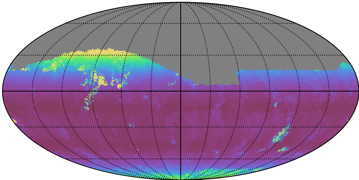
early_u_fpextra4.0_v3.4_10yrs Yr 1 i band: Median airmass
