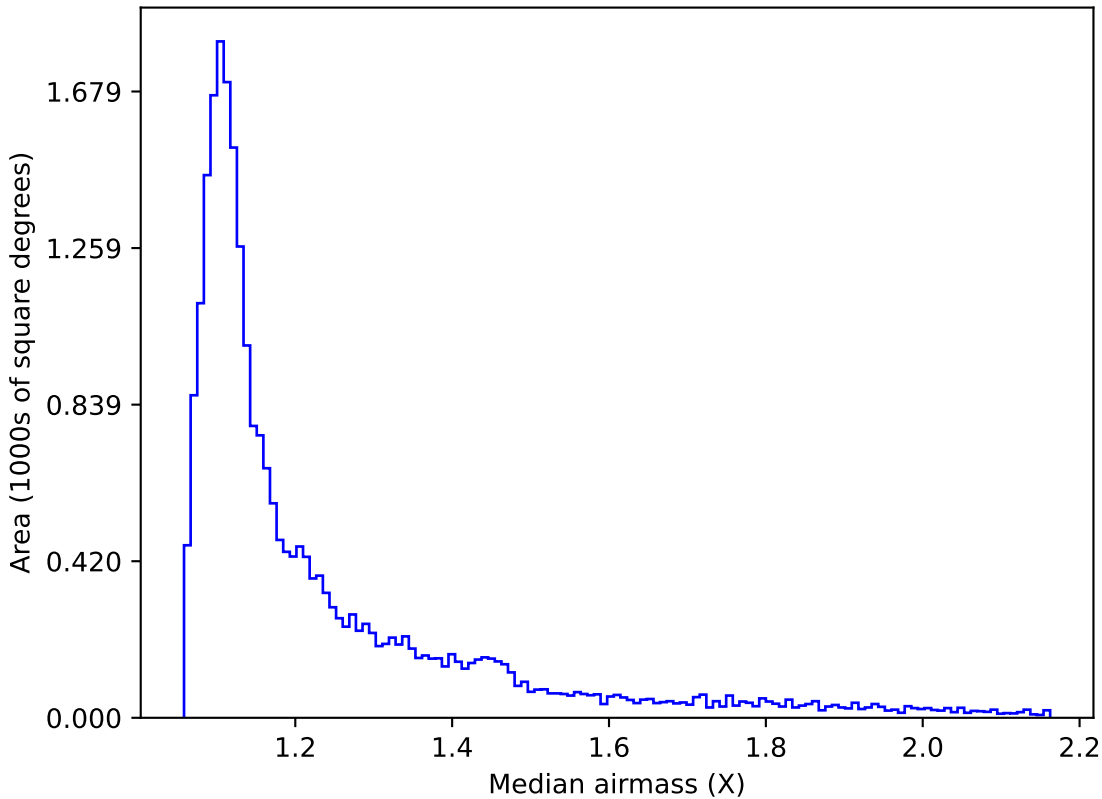
early_u_fpextra4.0_v3.4_10yrs Yr 1 i band: Median airmass
