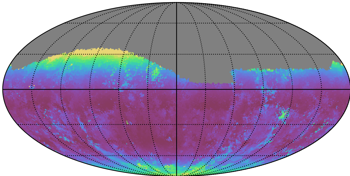
early_u_fpextra4.0_v3.4_10yrs Yr 1 g band: Median airmass
