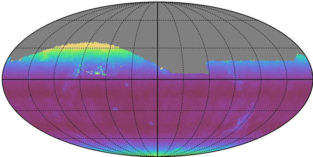
early_u_fpextra4.0_v3.4_10yrs Yr 1 all bands: Median airmass
