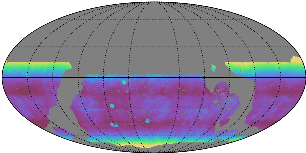
early_u_fpextra4.0_v3.4_10yrs WFD z band: Median airmass
