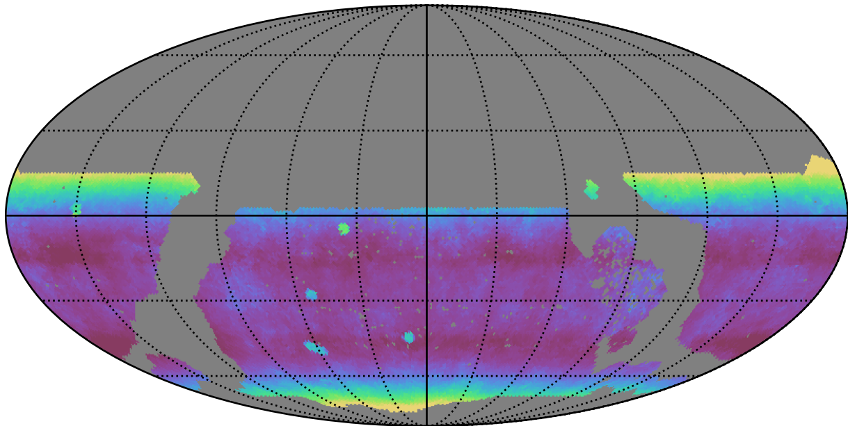
early_u_fpextra4.0_v3.4_10yrs WFD y band: Median airmass
