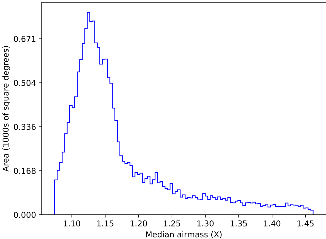
early_u_fpextra4.0_v3.4_10yrs WFD r band: Median airmass
