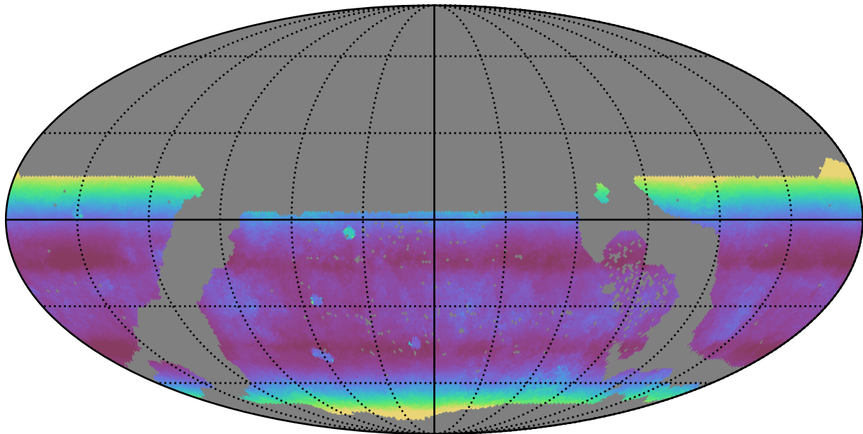
early_u_fpextra4.0_v3.4_10yrs WFD i band: Median airmass
