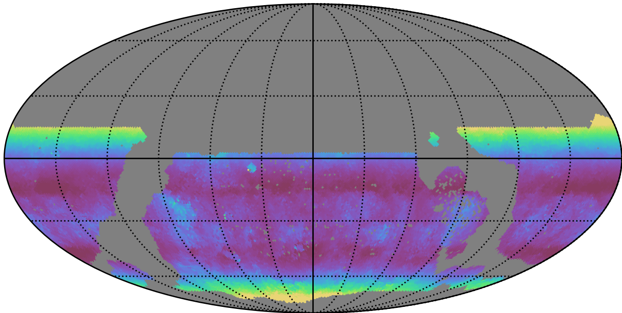
early_u_fpextra4.0_v3.4_10yrs WFD g band: Median airmass
