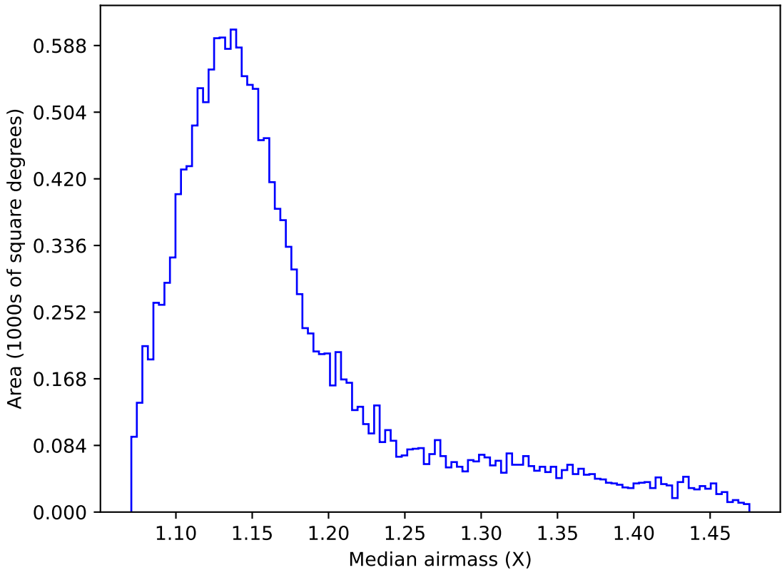
early_u_fpextra4.0_v3.4_10yrs WFD g band: Median airmass
