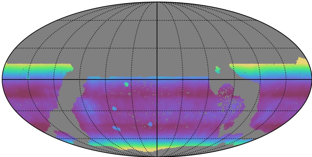
early_u_fpextra4.0_v3.4_10yrs WFD all bands: Median airmass
