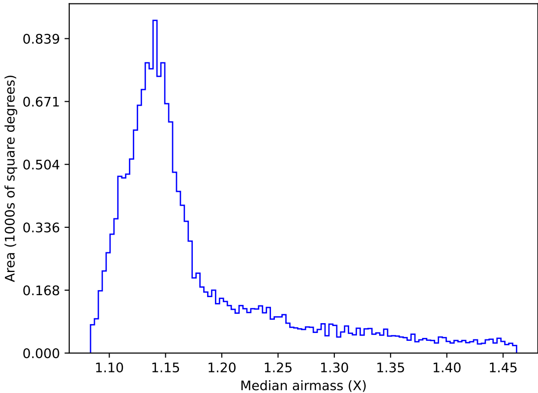
early_u_fpextra4.0_v3.4_10yrs WFD all bands: Median airmass
