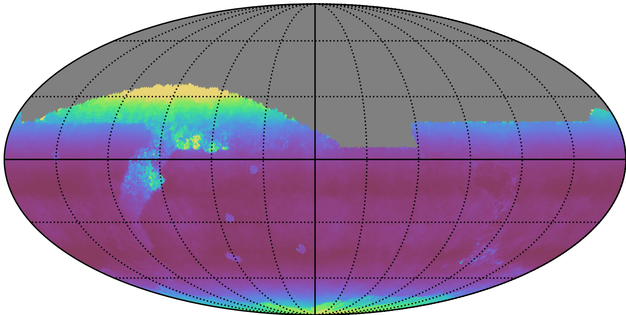
early_u_fpextra4.0_v3.4_10yrs All sky z band: Median airmass
