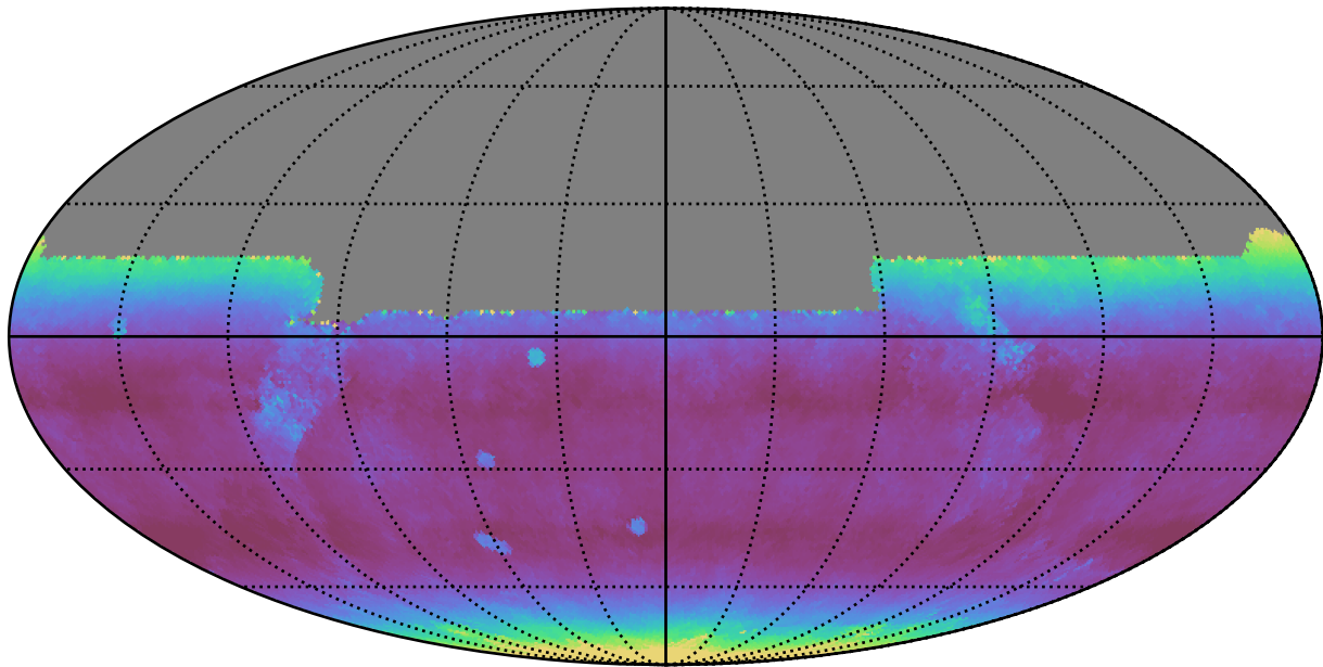
early_u_fpextra4.0_v3.4_10yrs All sky y band: Median airmass
