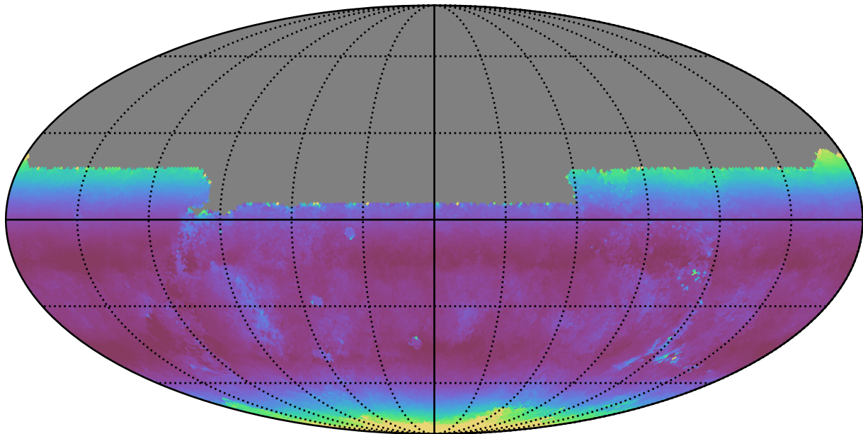
early_u_fpextra4.0_v3.4_10yrs All sky u band: Median airmass
