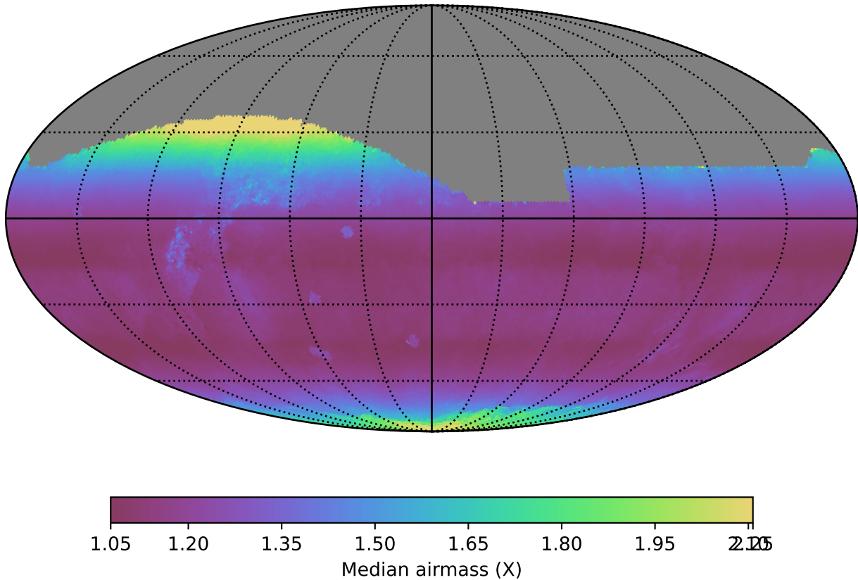
early_u_fpextra4.0_v3.4_10yrs All sky r band: Median airmass
